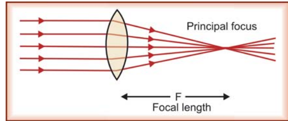
Fig. 4.11: Principal focus of a convex lens
