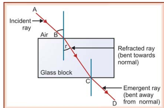
Fig. 4.7: Refraction through parallel sided slab of glass
