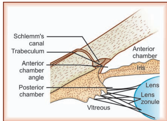
Fig. 15.1: Anatomy of the anterior chamber and its angle
