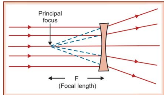
Fig. 4.12: Principal focus of a concave lens
